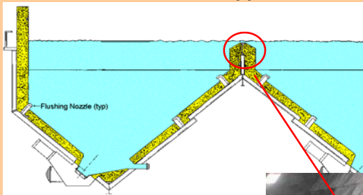
Stainless Steel Cricket Being Added To Existing Wet-Bottom Ash Hopper
